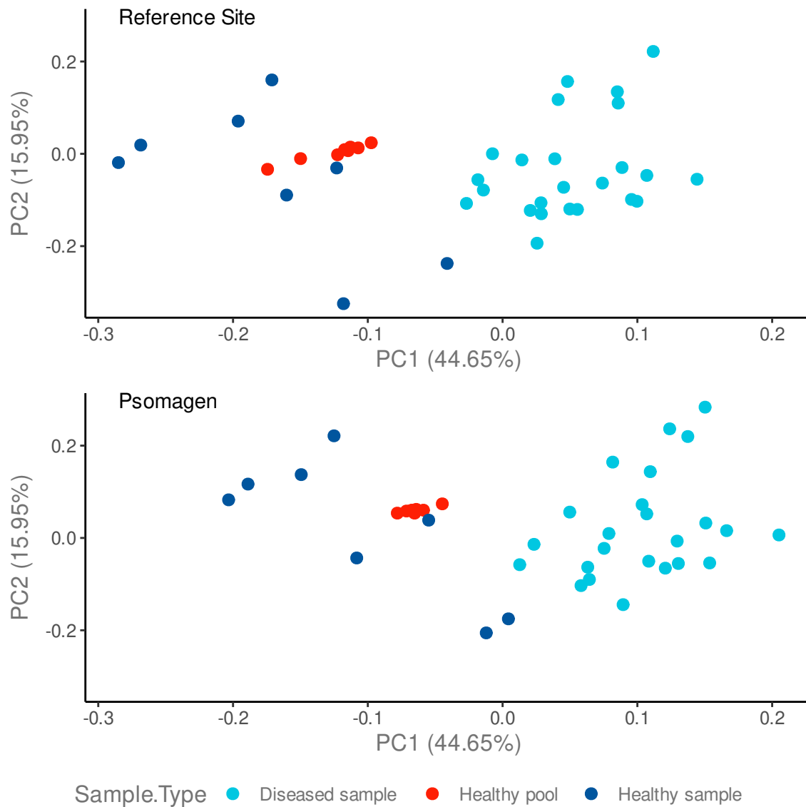
Figure 1: Separated PCA plots of data from Reference Site and Psomagen, colored by sample type. Each point represents one sample. The position of the point is based on all measured protein values. The percentages displayed show the percentage of explained variance per principal component.
